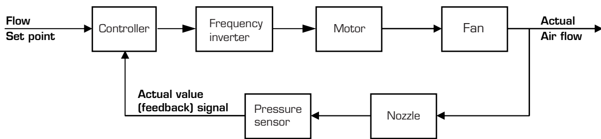
Flow control
