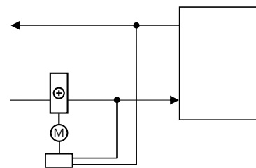
Basic diagram showing the extract air control principle
