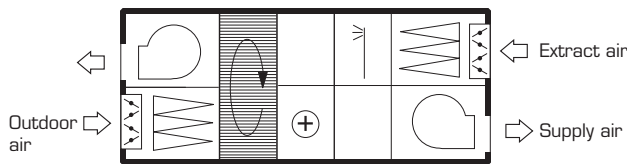
Extract air humidification
