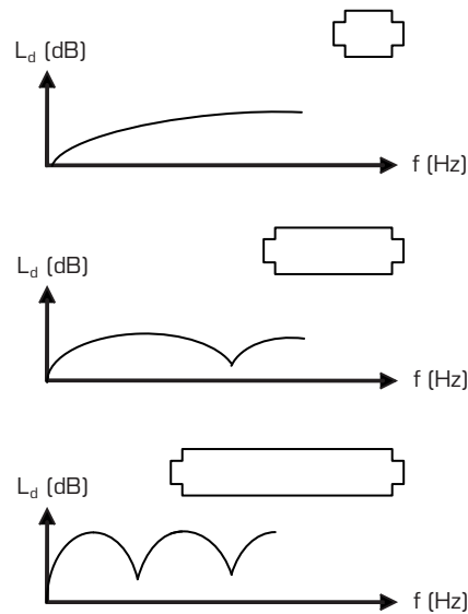
Increasing the length of the sound absorber increases the sound attenuation ( L_d ) in the lower frequencies but introduces resonances.
